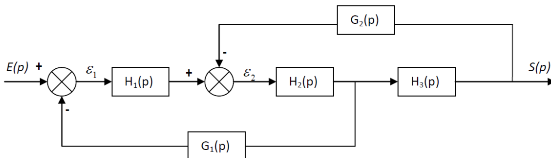
FIGURE 1 – Schéma-Bloc
